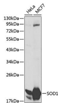
Fig. 1. Western blot analysis of extracts of various cell lines, using SOD1 antibody at 1:10000 dilution. Lysates/proteins: 25µg per lane. Blocking buffer: QuickBlock™ Blocking Buffer (P0231).
